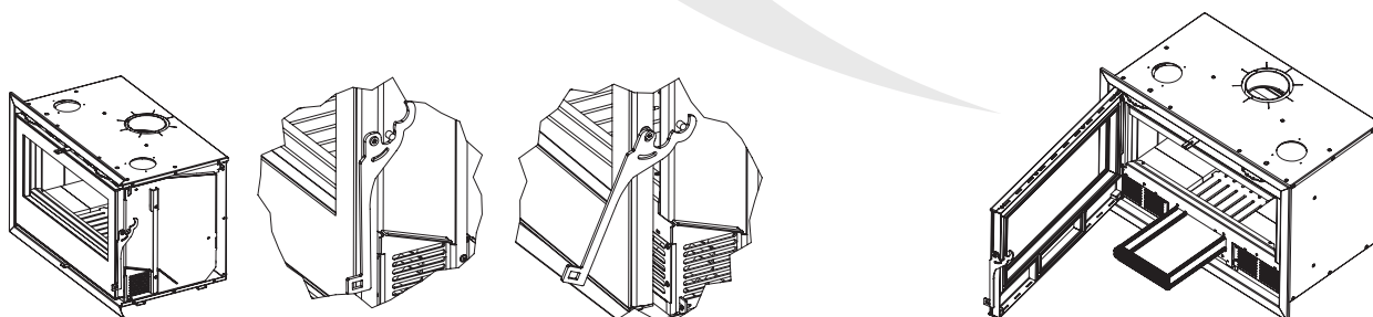
Ash pan in GALAXY/TAURUS/FUJI/TEIDE (R)
