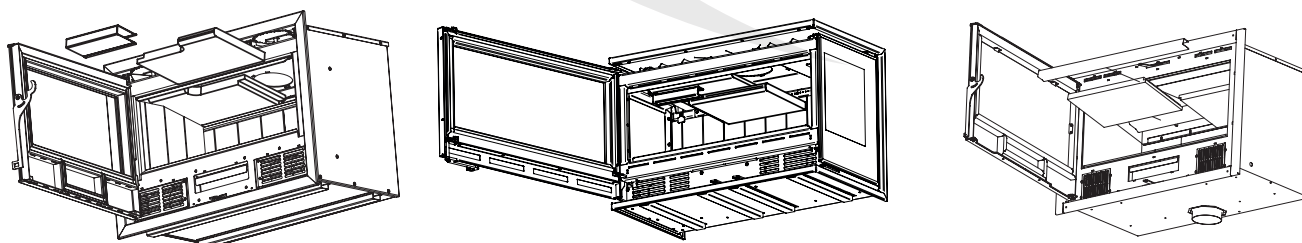
Disassembly of vermiculite deflector on GALAXY/TAURUS, PANORAMIC and TEIDE/FUJI devices.
