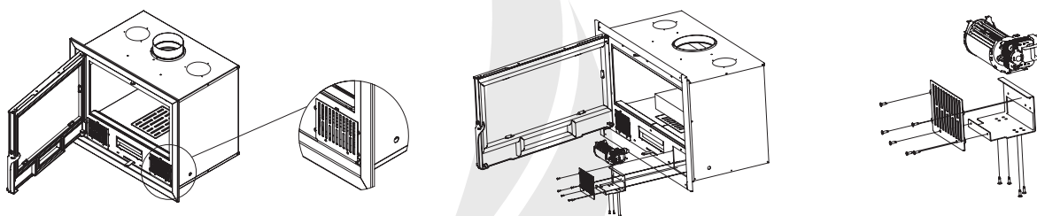
Replacement of the turbines in the FUJI /TEIDE insertable devices
