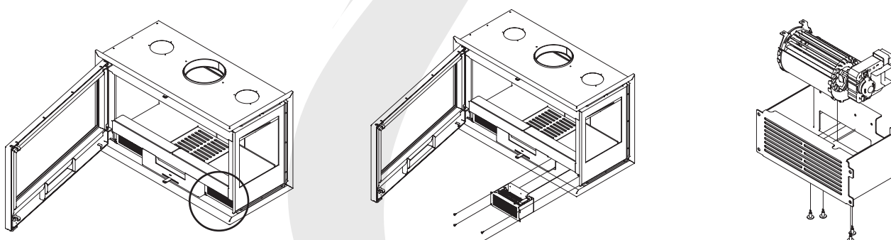
Replacement of the turbines in the F series and PANORAMIC devices
