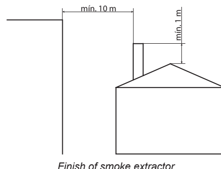
Finish of smoke extractor
